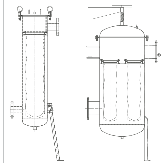
Single Bag Filter
